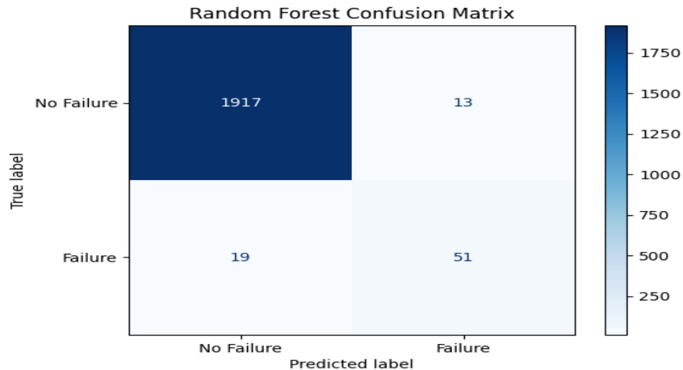
Figure 7 Confusion Matrix
