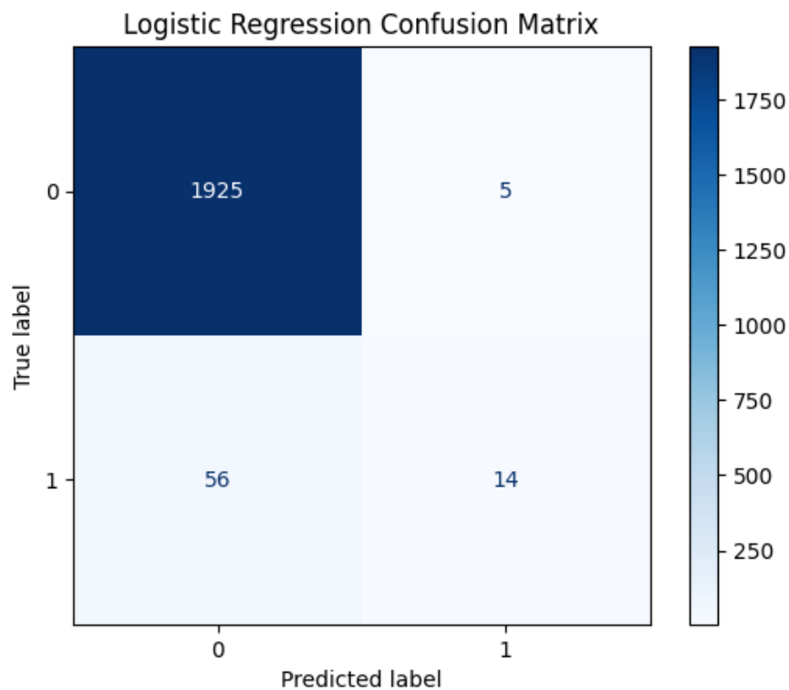
Figure 13 Confusion Matrix
