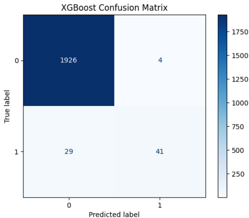
Figure 9 Confusion Matrix
