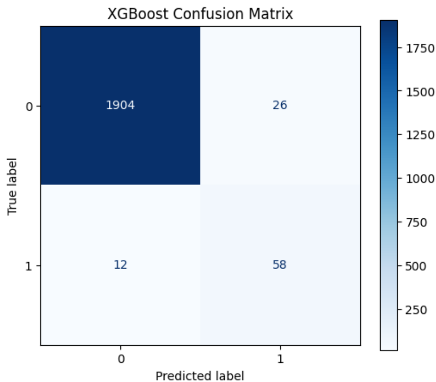
Figure 16 Confusion Matrix
