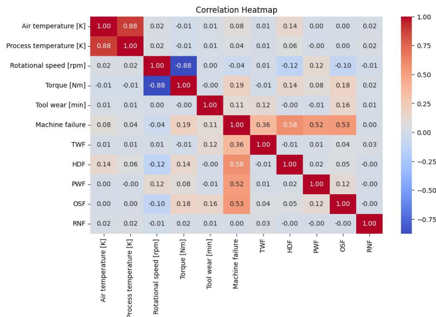
Figure 2 Correlation Heatmap
