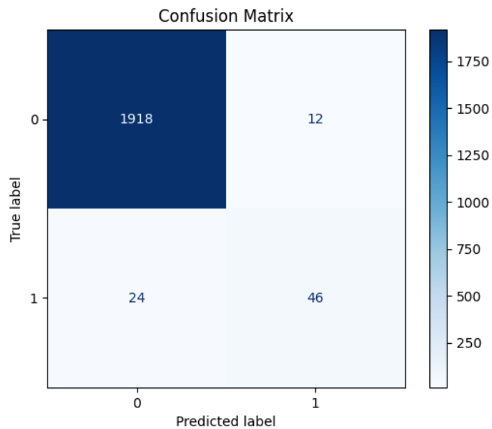
Figure 22 Confusion Matrix
