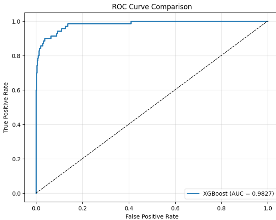
Figure 17 XG BOOST
