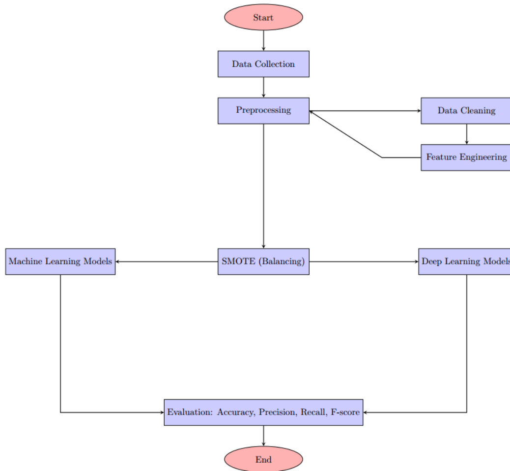
Figure 1 Proposed Flowchart
