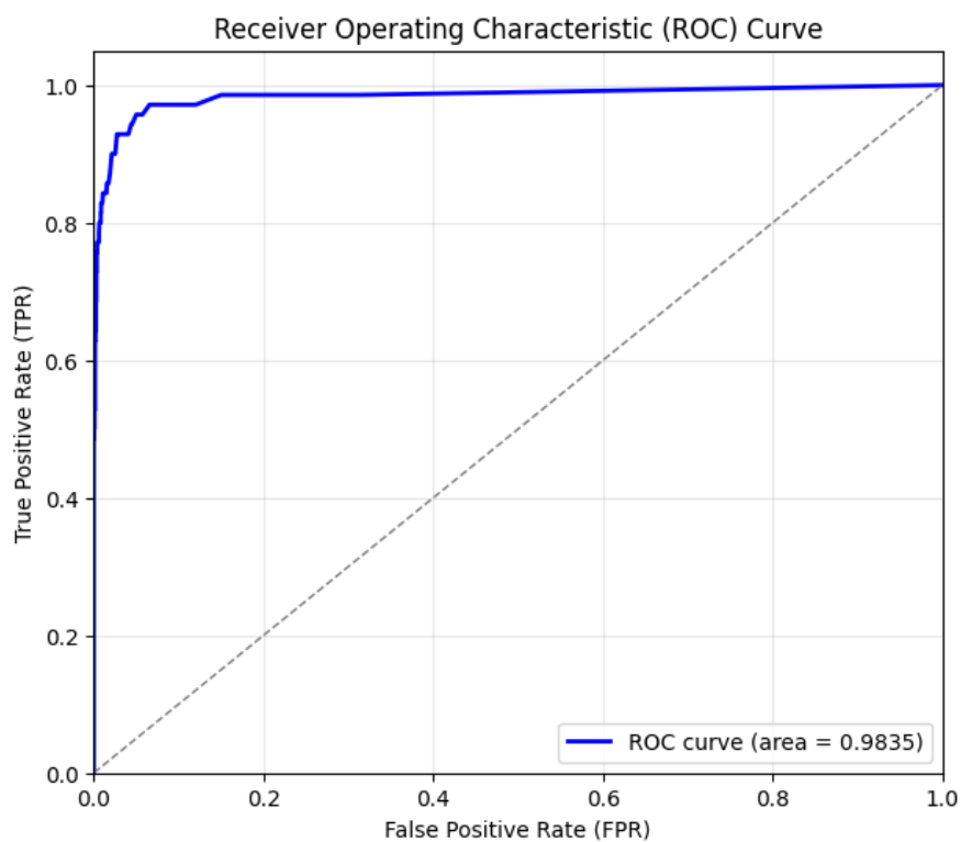
Figure 8 RANDOM FOREST
