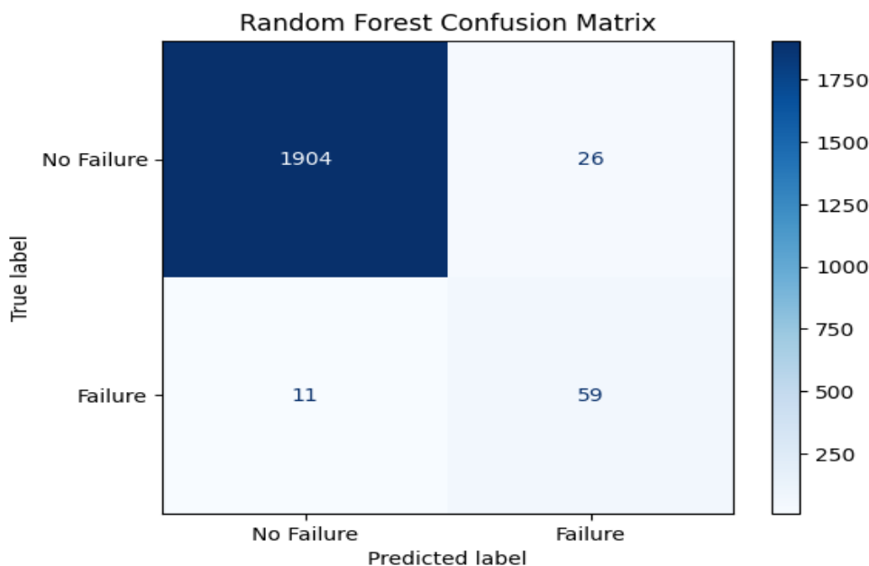
Figure 14 Confusion Matrix
