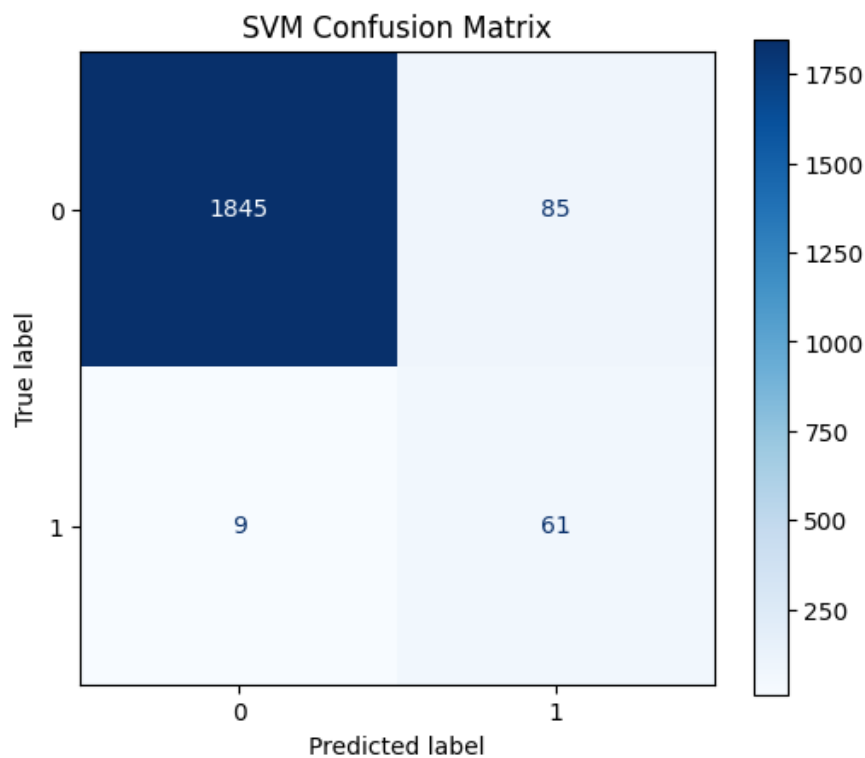
Figure 18 Confusion Matrix
