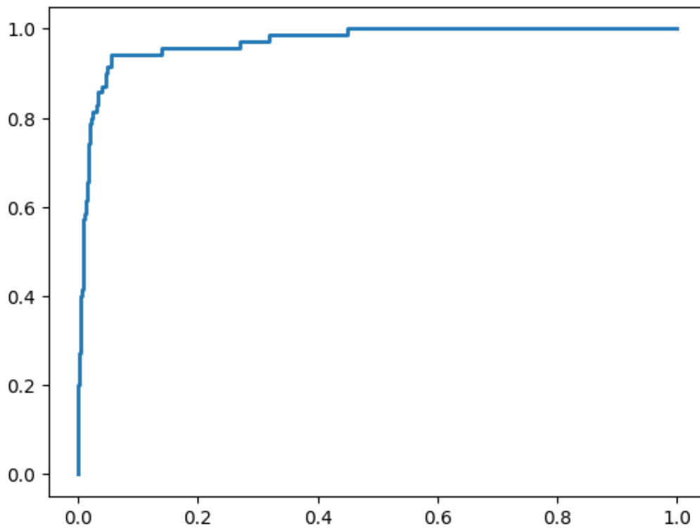
Figure 19 svm
