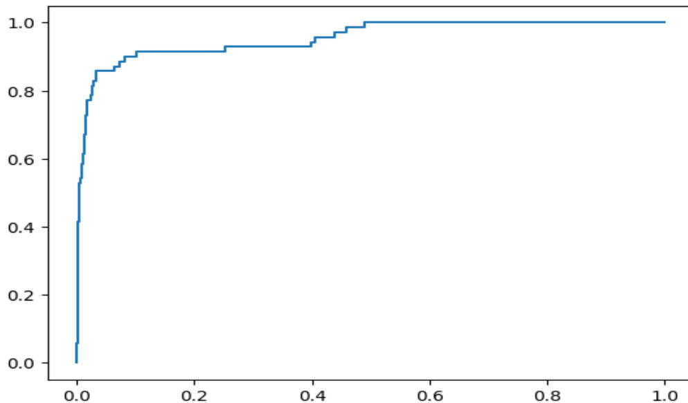
Figure 12 SVM
