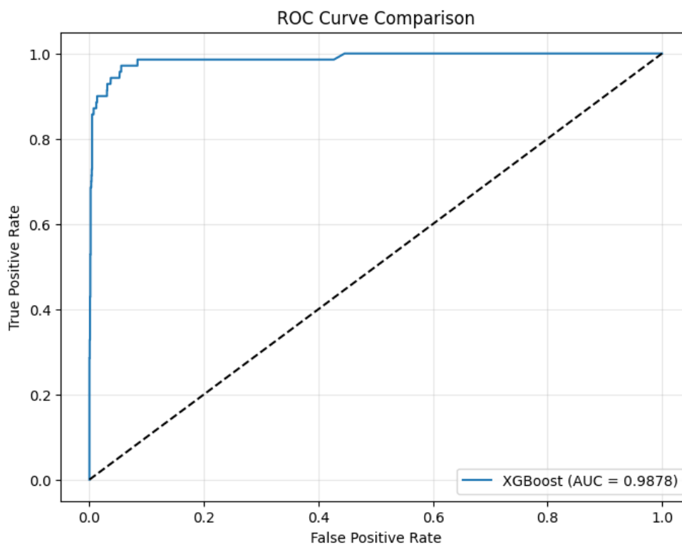
Figure 10 XGBOOST
