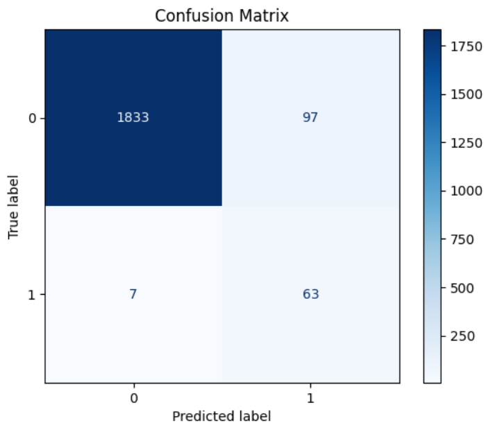
Figure 25 Confusion Matrix
