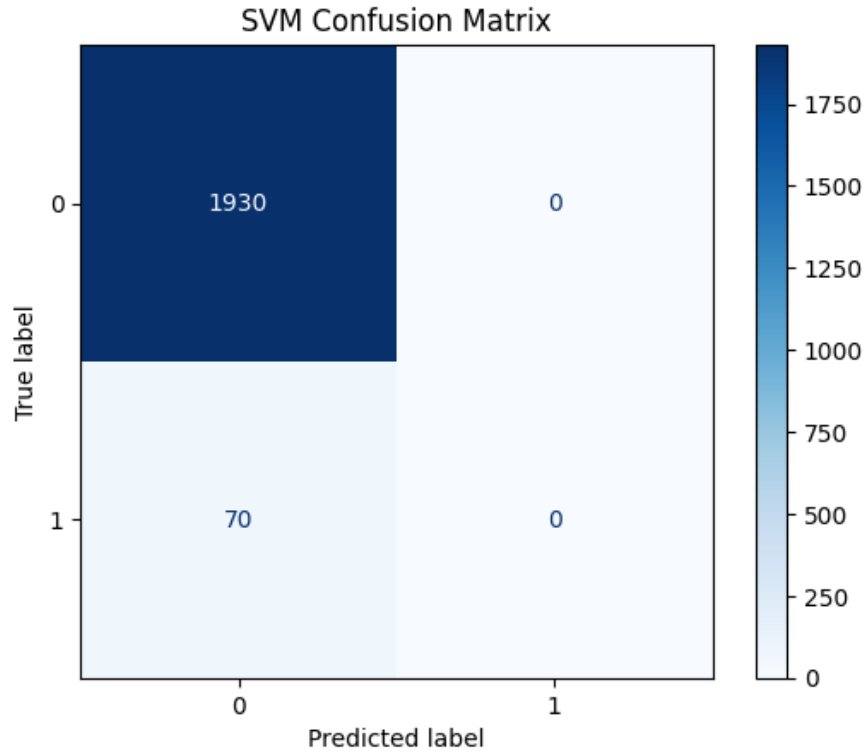
Figure 11 Confusion Matrix
