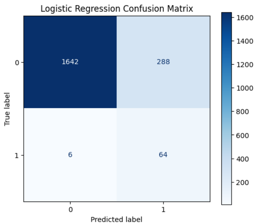
Figure 20 Confusion Matrix
