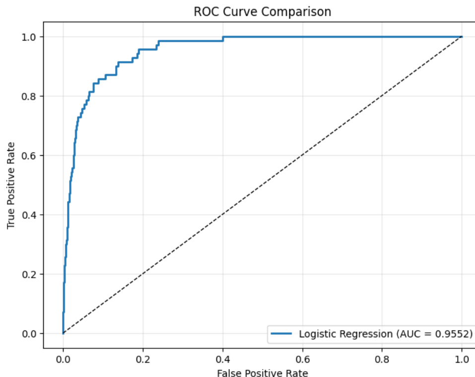
Figure 21 logistic regression
