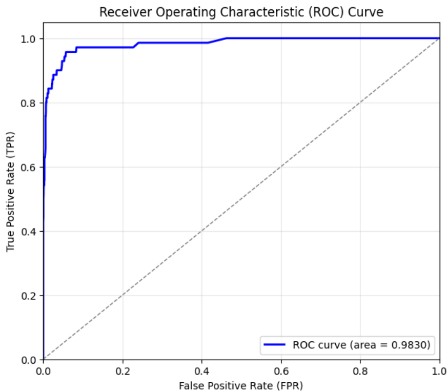
Figure 15 RANDOM FOREST
