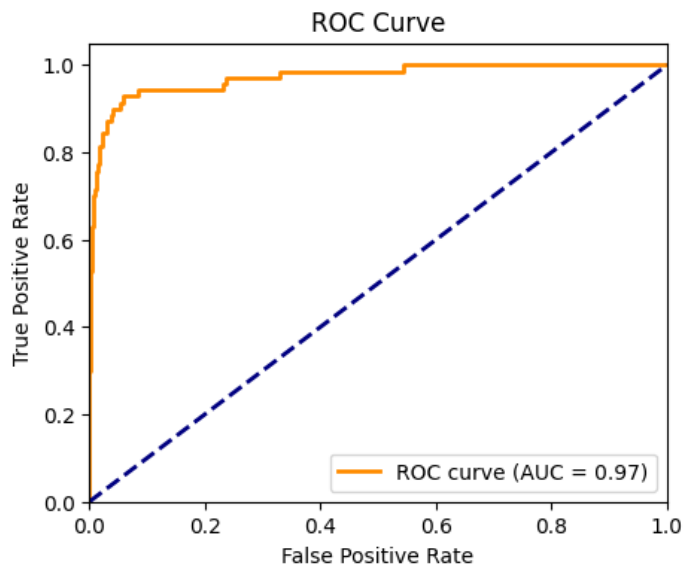
Figure 24 Conv1D With SMOTE
